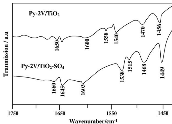
Fig. 6. In situ FT-IR spectra in the 1400\text{--}1750\text{ cm}^{-1} range due to pyridine adsorption at room temperature. The spectra were recorded after evacuation for 10\text{ min} at 300\text{ K} .
